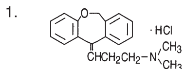
Doxepin hydrochloride
