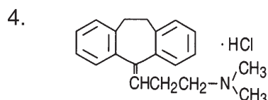
Amitriptyline hydrochloride
