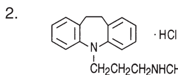
Desipramine hydrochloride
