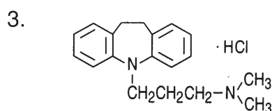
Imipramine hydrochloride
